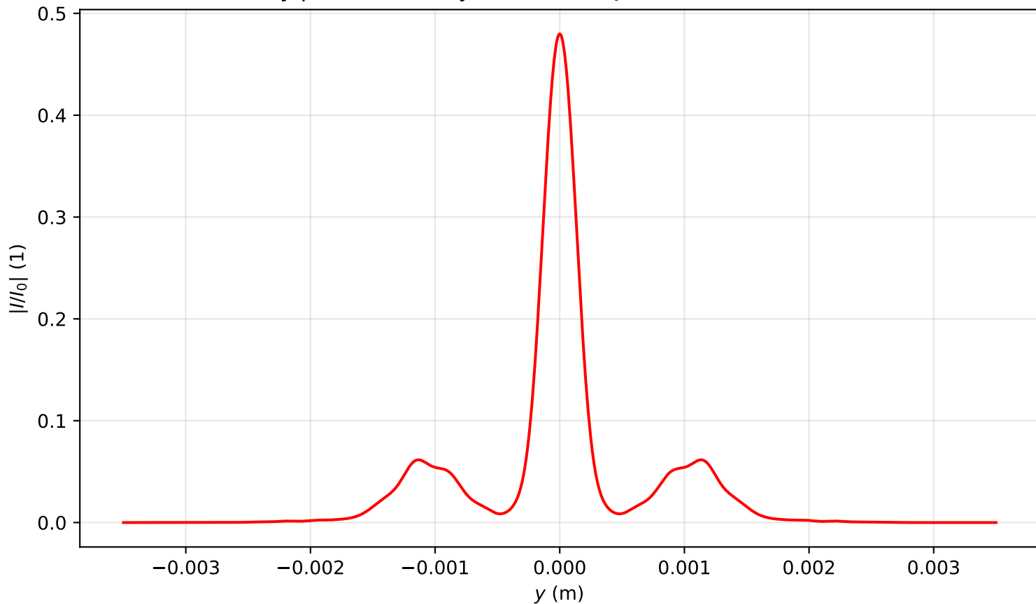
Intensity profile I(x = 0, y, z = 2.627)/I_0 , P_{in}=8.5P_{cr} , artificial time
